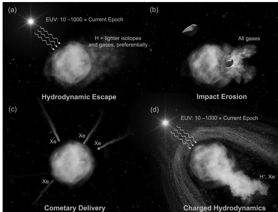
Fig. 5. See Plate 33 for color version. Schematics showing major features of the four main hypotheses of early planetary evolution that led to atmospheric Xe-isotopic abundances on the terrestrial planets. (a) Hydrodynamic escape. Early solar EUV was 100–1000 times more intense than today, heating the atmosphere to the point where H began to flow out of the exosphere. It dragged lighter molecules with it, fractionating the atmosphere so that it was isotopically heavier. (b) Impact erosion. Small impacts both added material and eroded the atmosphere. Large impacts blew off most of the atmosphere above the plane of impact, indiscriminate of mass, so no fractionation occurred. (c) Cometary delivery. Cold comets from the outer solar system with trapped Xe incorporating the isotopic ratios of the cold outer solar system impacted the surface. (d) Charged hydrodynamics. Hydrogen and Xe are both easily ionized, unlike other molecules. Thus ionization by the UV or solar wind preferentially allowed H and Xe to escape, while also allowing somewhat smaller portions of other ionized atoms and molecules to go along for the ride. The process is fractionating, dependent upon both mass and ionization energy.
