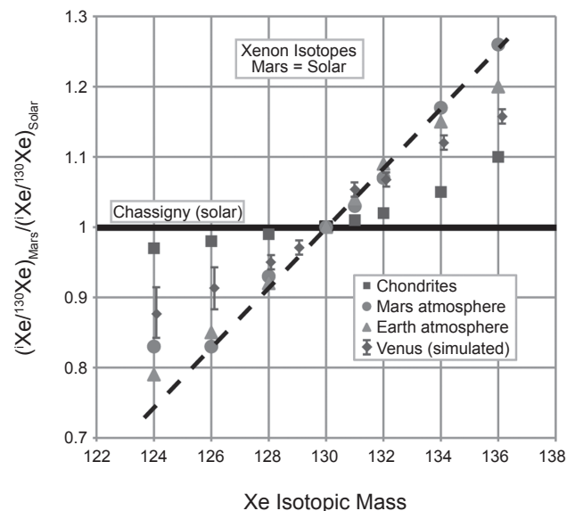
Fig. 3. See Plate 31 for color version. Fractionation of Xe isotopes. Possible Venus Xe fractionation pattern observed by a future in situ mission is depicted (green) compared to the patterns of Earth, Mars, chondrites, and the Sun (after Bogard et al., 2001). A common Venus/Earth/Mars pattern would bolster the hypothesis that a common source of comets or large planetesimals delivered volatiles throughout the inner solar system. A different pattern for Venus would strengthen the solar EUV blowoff theory.
