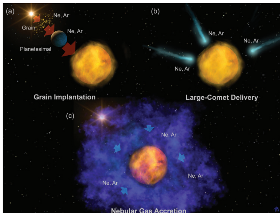
Plate 34. Schematics of the three main hypotheses for the origin of large Ne and Ar abundances in Venus's atmosphere. (a) Grain implantation. Early solar wind fluxes were many orders of magnitude higher than today. Solar-wind Ar and Ne implanted into grains around the Sun, which coalesced into Ar,Ne-rich planetesimals that impacted Venus. (b) Large-comet delivery. Argon and Ne frozen and trapped in cometary ice lattices was delivered by one or more large comets ( \geq 200 km diameter) from the cold reaches of the outer solar system, leaving Venus with an Ar,Ne-rich atmosphere. (c) Nebular gas. Venus' present atmosphere came directly from the nebula in which it was formed. The atmosphere survived relatively intact against subsequent impactors that blew off the original atmospheres of Earth and Mars, resulting in a relatively Ar,Ne-rich atmosphere on Venus.
