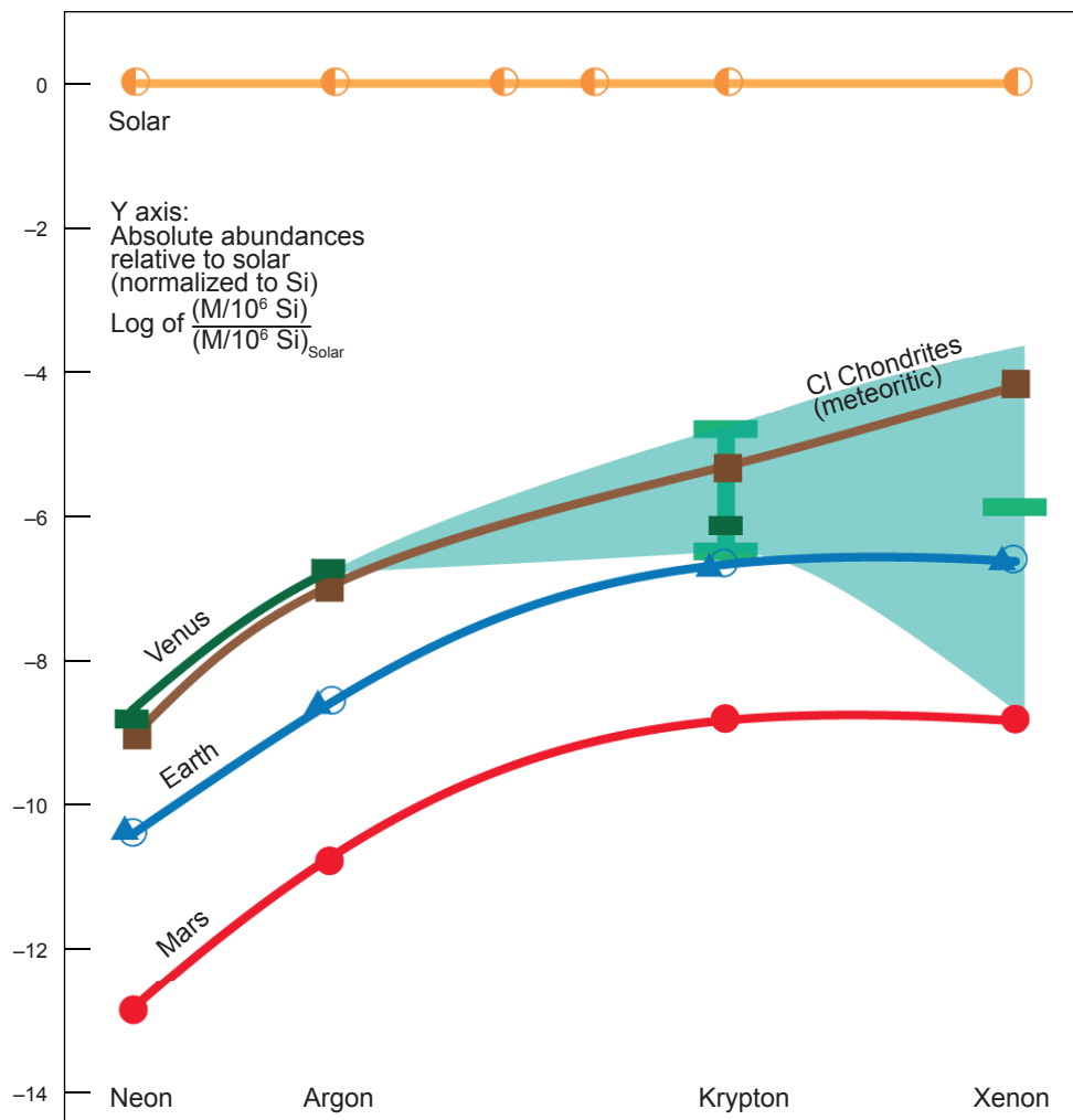
Plate 32. Noble gas abundances for Earth, Mars, Venus, chondrites, and the Sun (after Pepin , 1991). Missing Xe and poorly constrained Kr data for Venus are critical for understanding the history of its early atmosphere. For Ne and Ar, and likely Kr, Venus is more enhanced in noble gases vs. Earth and Mars, likely indicating (1) a large blowoff of the original atmospheres of Mars and Earth, and/or (2) enhanced delivery of noble elements to Venus from comets and/or solar-wind-implanted planetesimals. For Venus, the unknown/poorly constrained Xe/Kr and Kr/Ar ratios — denoted by the range of slopes of the aqua area — are consistent with all solar system objects shown, including (1) a solar-type (Jupiter and cometary) composition (orange line), (2) a chondritic composition (brown line), and (3) the composition of Earth and Mars (blue and red lines).
