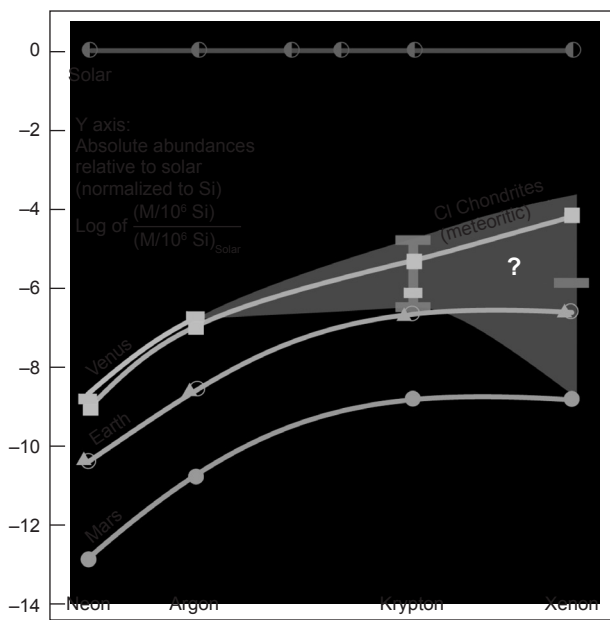
Fig. 4. See Plate 32 for color version. Noble gas abundances for Earth, Mars, Venus, chondrites, and the Sun (after Pepin, 1991 ). Missing Xe and poorly constrained Kr data for Venus are critical for understanding the history of its early atmosphere. For Ne and Ar, and likely Kr, Venus is more enhanced in noble gases vs. Earth and Mars, likely indicating (1) a large blowoff of the original atmospheres of Mars and Earth, and/or (2) enhanced delivery of noble elements to Venus from comets and/or solar-wind-implanted planetesimals. For Venus, the unknown/poorly constrained Xe/Kr and Kr/Ar ratios — denoted by the range of slopes of the aqua area — are consistent with all solar system objects shown, including (1) a solar-type (Jupiter and cometary) composition (orange line), (2) a chondritic composition (brown line), and (3) the composition of Earth and Mars (blue and red lines).
