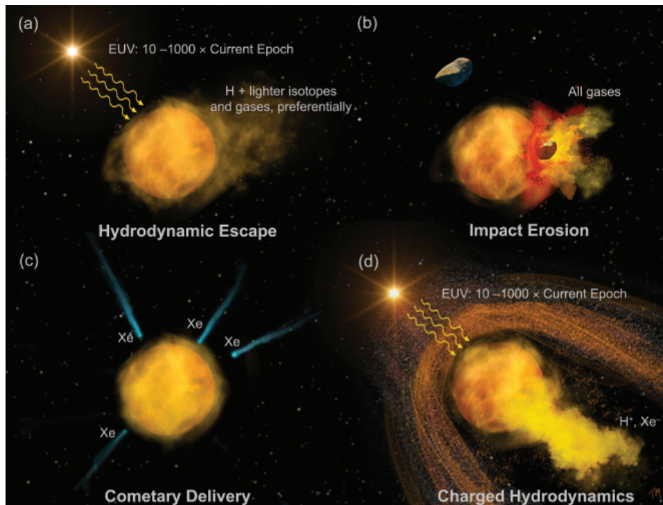
Plate 33. Schematics showing major features of the four main hypotheses of early planetary evolution that led to atmospheric Xe-isotopic abundances on the terrestrial planets. (a) Hydrodynamic escape. Early solar EUV was 100–1000 times more intense than today, heating the atmosphere to the point where H began to flow out of the exosphere. It dragged lighter molecules with it, fractionating the atmosphere so that it was isotopically heavier. (b) Impact erosion. Small impacts both added material and eroded the atmosphere. Large impacts blew off most of the atmosphere above the plane of impact, indiscriminate of mass, so no fractionation occurred. (c) Cometary delivery. Cold comets from the outer solar system with trapped Xe incorporating the isotopic ratios of the cold outer solar system impacted the surface. (d) Charged hydrodynamics. Hydrogen and Xe are both easily ionized, unlike other molecules. Thus ionization by the UV or solar wind preferentially allowed H and Xe to escape, while also allowing somewhat smaller portions of other ionized atoms and molecules to go along for the ride. The process is fractionating, dependent upon both mass and ionization energy.
