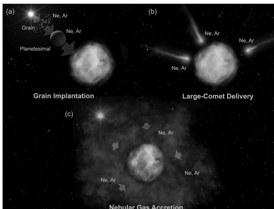
Fig. 6. See Plate 34 for color version. Schematics of the three main hypotheses for the origin of large Ne and Ar abundances in Venus' atmosphere. (a) Grain implantation. Early solar wind fluxes were many orders of magnitude higher than today. Solar-wind Ar and Ne implanted into grains around the Sun, which coalesced into Ar,Ne-rich planetesimals that impacted Venus. (b) Large-comet delivery. Argon and Ne frozen and trapped in cometary ice lattices was delivered by one or more large comets ( \geq 200 km diameter) from the cold reaches of the outer solar system, leaving Venus with an Ar,Ne-rich atmosphere. (c) Nebular gas. Venus' present atmosphere came directly from the nebula in which it was formed. The atmosphere survived relatively intact against subsequent impactors that blew off the original atmospheres of Earth and Mars, resulting in a relatively Ar,Ne-rich atmosphere on Venus.
