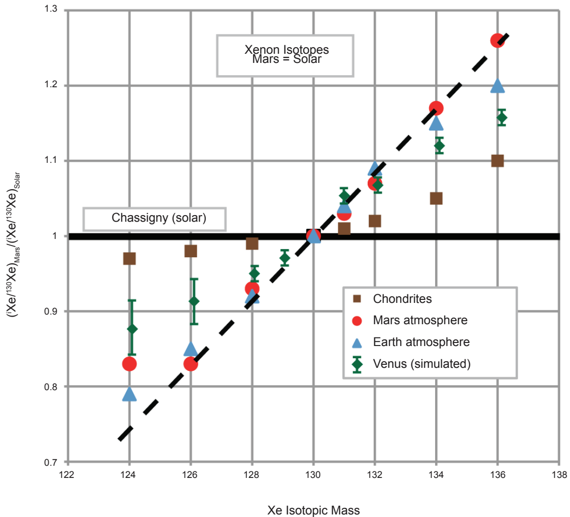
Plate 31. Fractionation of Xe isotopes. Possible Venus Xe fractionation pattern observed by a future in situ mission is depicted (green) compared to the patterns of Earth, Mars, chondrites, and the Sun (after Bogard et al. , 2001). A common Venus/Earth/Mars pattern would bolster the hypothesis that a common source of comets or large planetesimals delivered volatiles throughout the inner solar system. A different pattern for Venus would strengthen the solar EUV blowoff theory.
